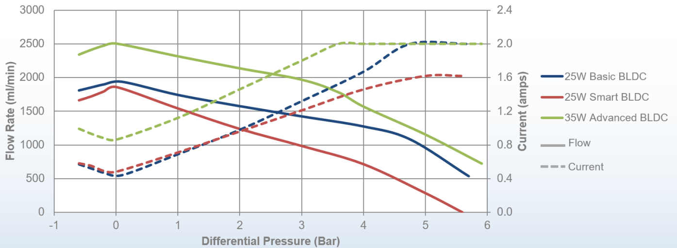
Cerotor 1500 Maximum Flow Curves (water)
