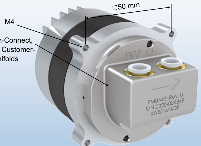
Advanced BLDC
